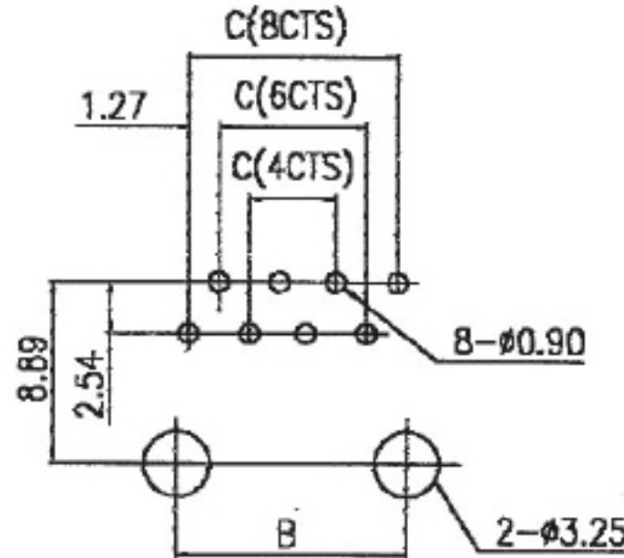
PCB Layout
