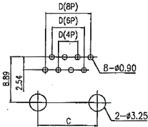
PCB Layout
