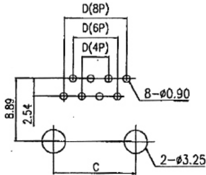
PCB Layout
