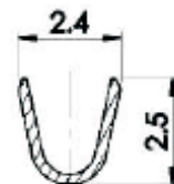
SEC. B-B'
