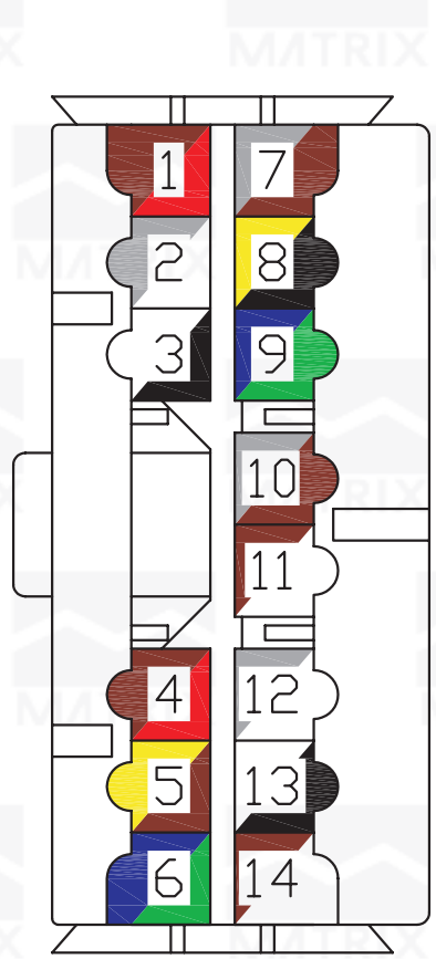
BACK SIGHT (SEEN OF THE WIRE)
