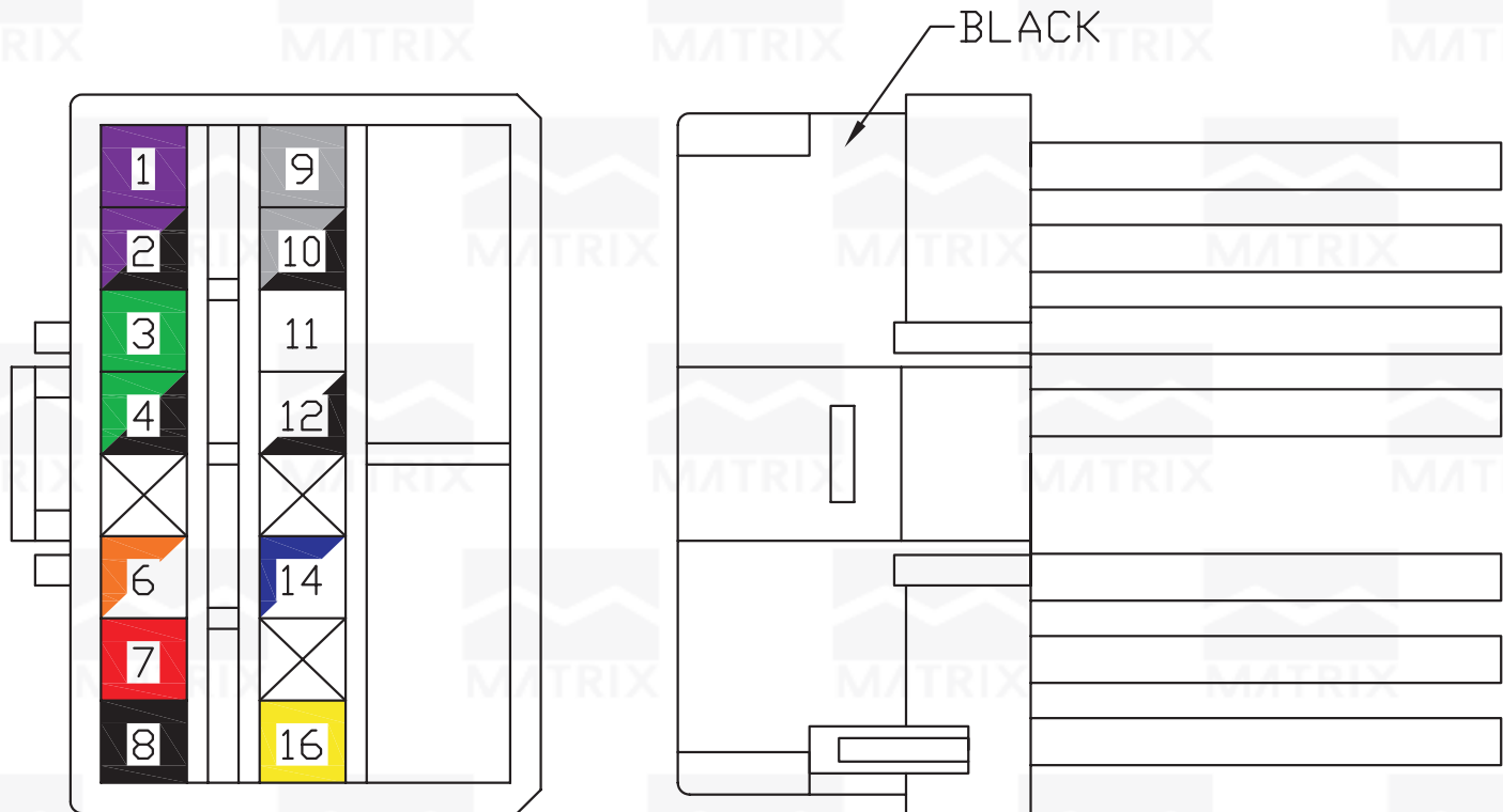
BACK SIGHT (SEEN OF THE WIRE)
