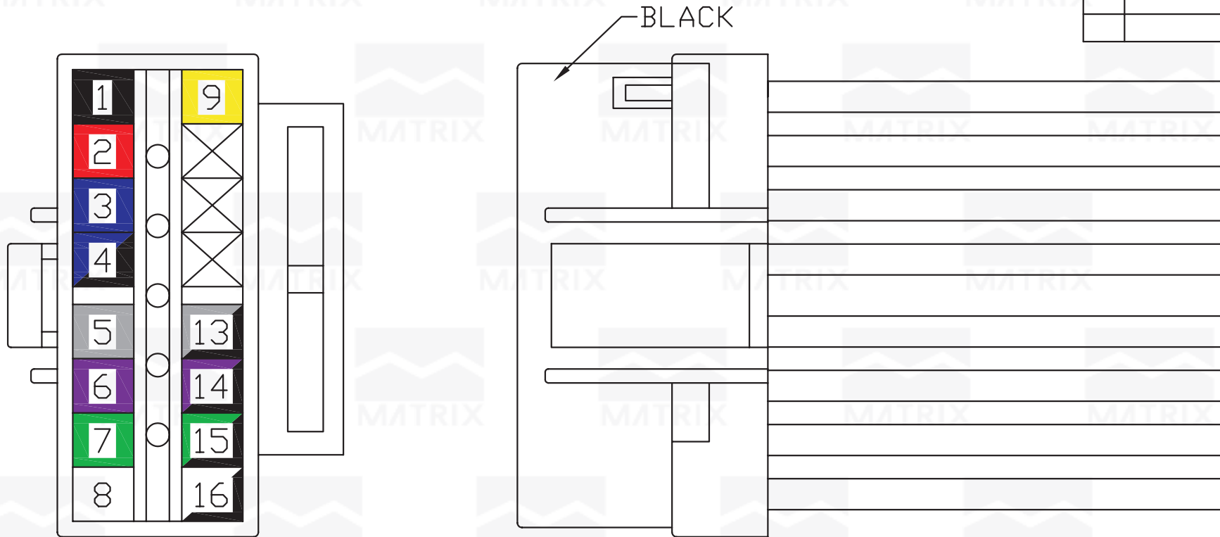
BACK SIGHT (SEEN OF THE WIRE)
