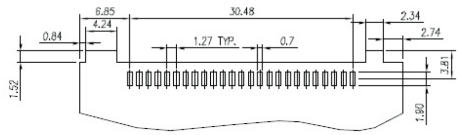
RECOMMENDED P.C.B. PATTERN
